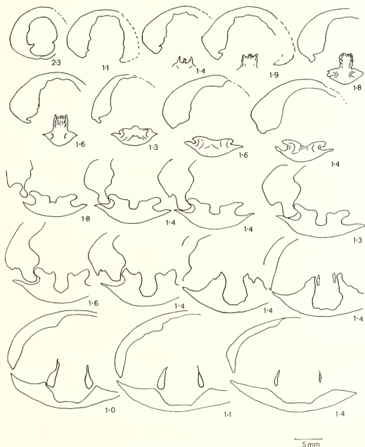
TEXT-FIG. 4. Twenty transverse serial sections through the umbo of a specimen of ' Carneithyris rockallensis sp. nov. obtained from a block of sandstone dredged from the north-western slope of Rockall Bank.
